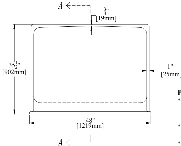
48" [1219mm] Dome for Models 5843, 5843X, 5843L/S or RS, 5843LX/S or RX/S, 5848, 5848X, 6843L/S or R/S, and 9648
